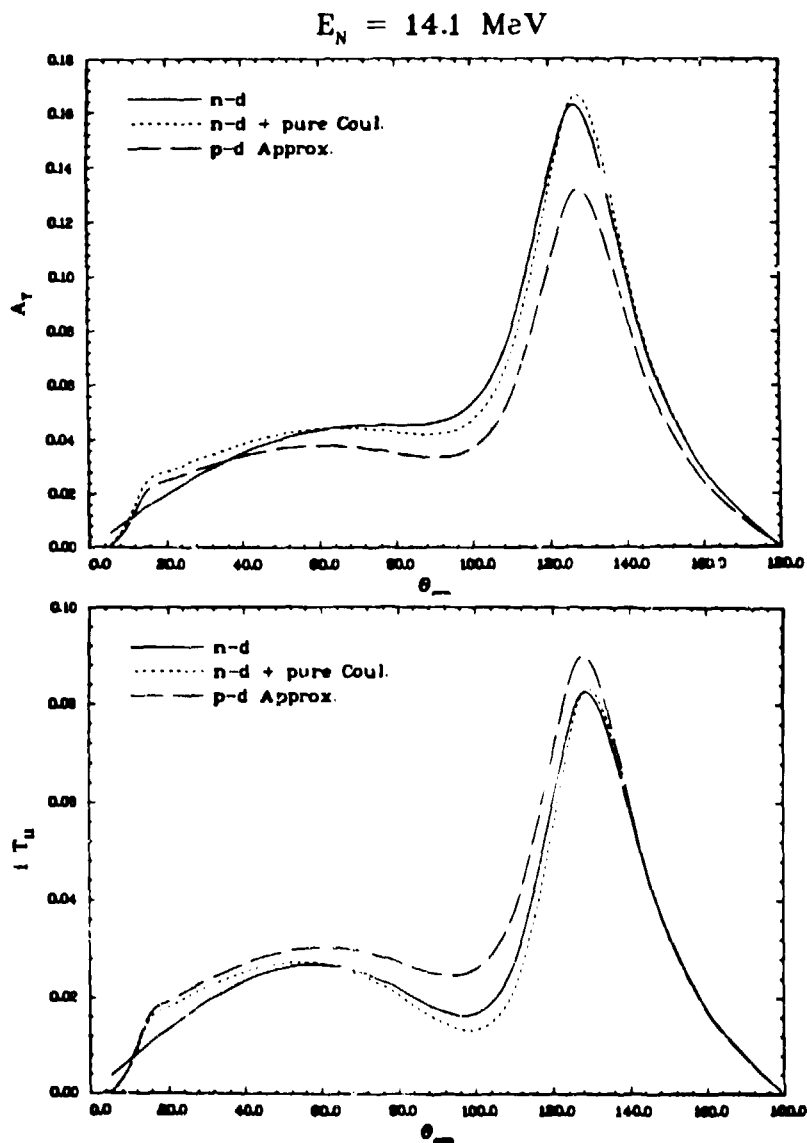
Fig. 2. Same as Fig. 1, but E_{Lab} = 14.1 \text{ MeV} .
