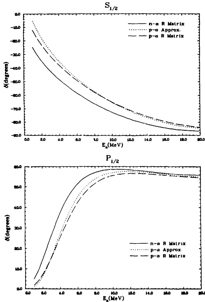
Fig. 4. Phase shifts for n- \alpha and p- \alpha scattering.
