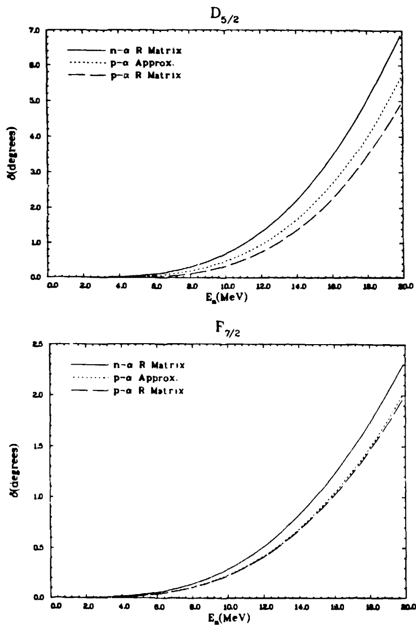
Fig. 5. Same as Fig. 4.
