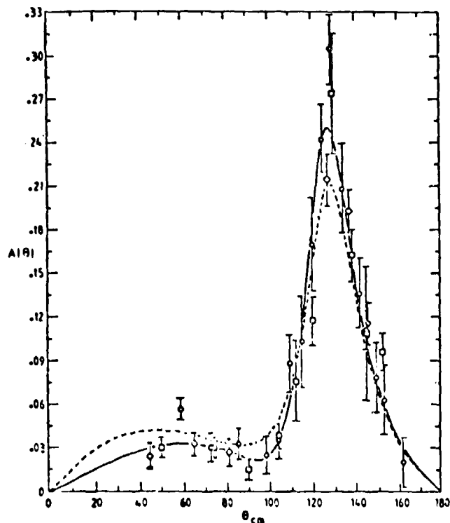
Fig. 3. Solid line is a fit to the n-d data and dashed line to the p-d data.
