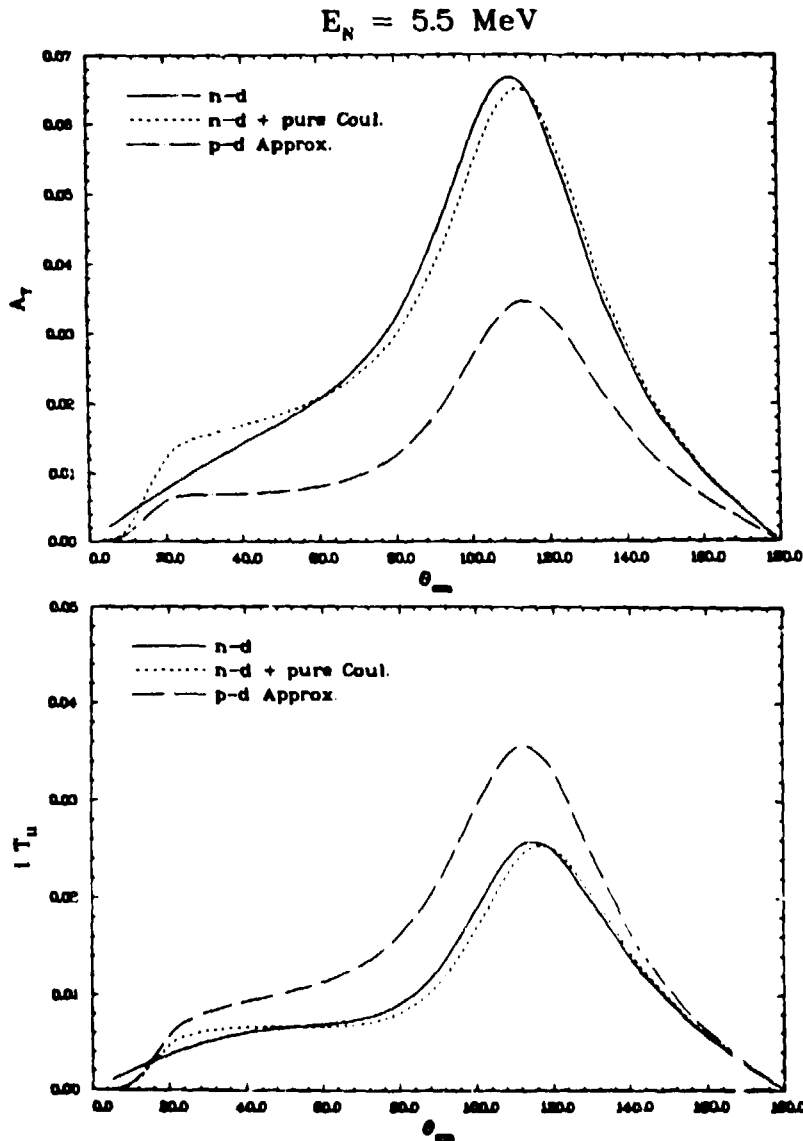
Fig. 1. Vector analyzing powers A_y and iT_{11} for elastic n-d and p-d scattering at E_{Lab} = 5.5 \text{ MeV} for the incident nucleon.
