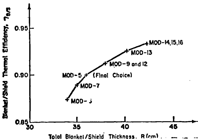
FIGURE 8. Thermal efficiencies for several optimized blanket/shield assemblies vs total B/S-thickness.
