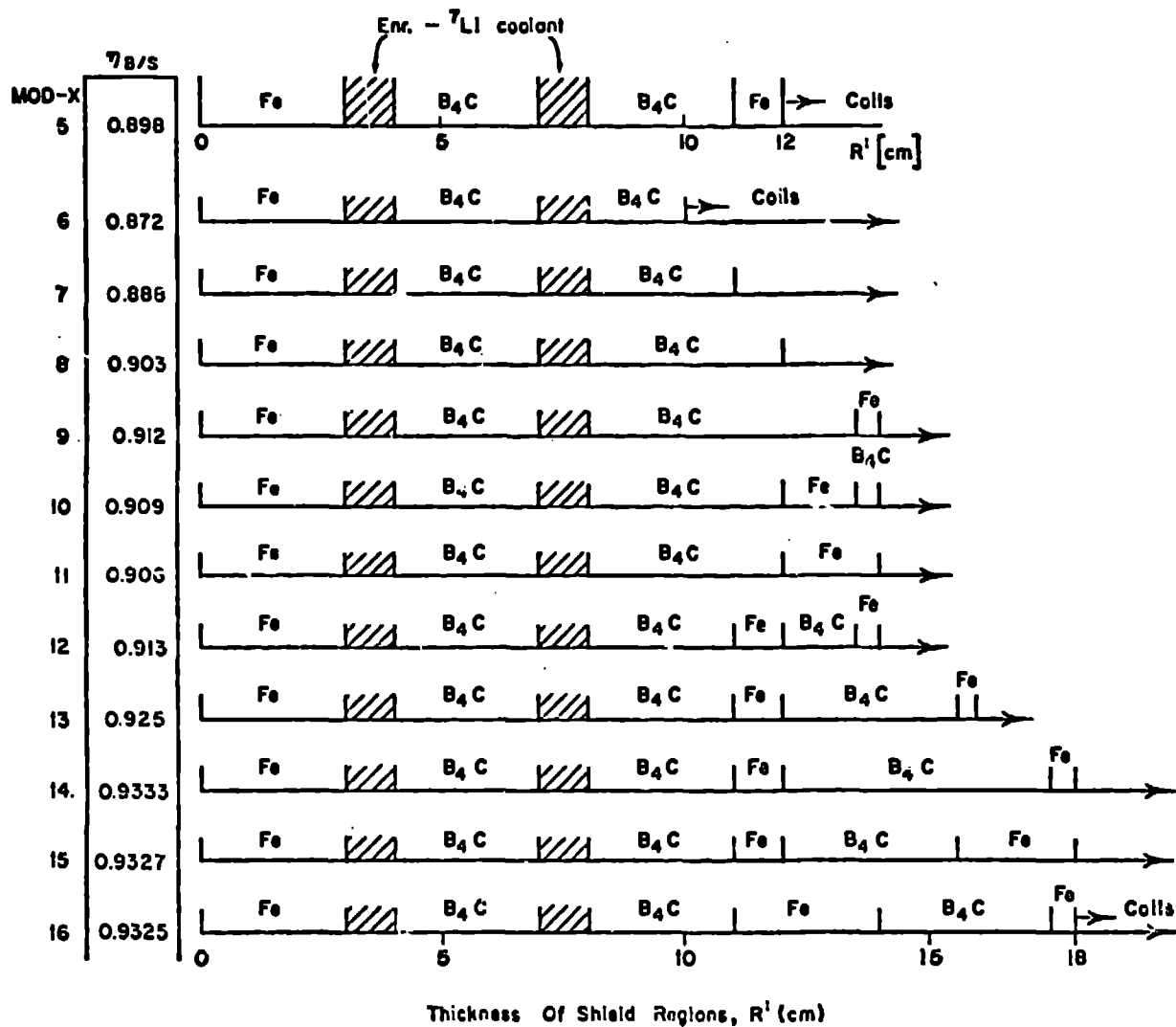
FIGURE 7. Schematic of optimized shield regions (MOD-5 is used in new RTPR blanket) with variations, indicating total blanket/shield thermal efficiencies \eta_{B/S} .
