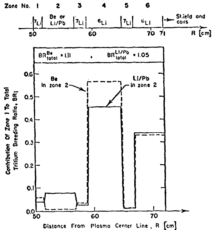
FIGURE 2. Breeding zones arrangement in MOD-2 blanket with contributions of individual zones to total tritium breeding for Be- and Li/Pb-multipliers.
