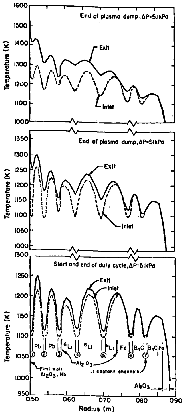
FIGURE 11. Radial temperature distributions throughout the optimized blanket/shield for varying plasma conditions.
