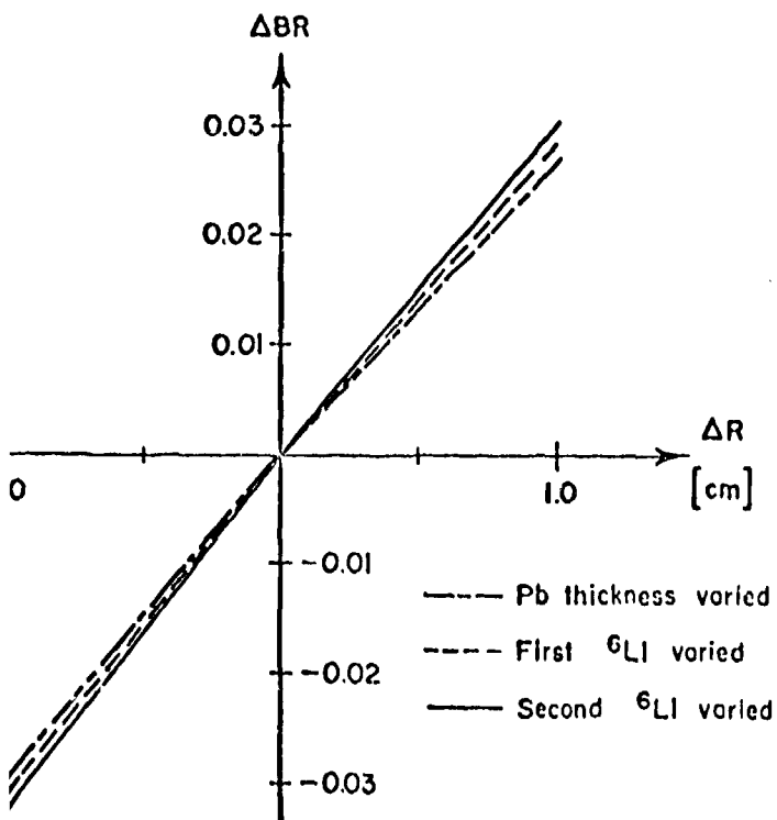
FIGURE 4. Sensitivity of total tritium breeding to zone thickness variations in MOD-2 blanket.
