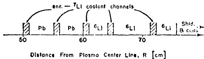
FIGURE 5. Schematic of breeding region of MOD-3 blanket.
