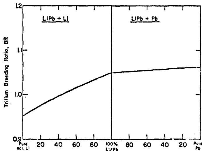
FIGURE 3. Variation of tritium breeding with varying composition of zone 2 in MOD-2 blanket.
