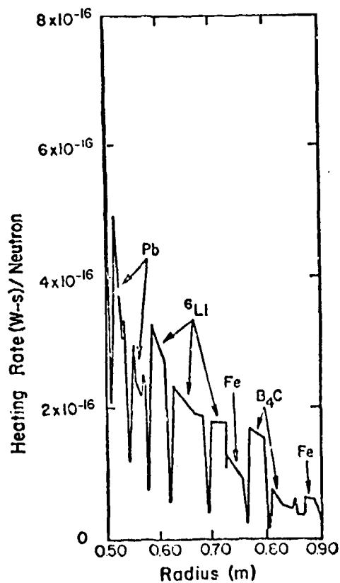
FIGURE 10. Radial distribution of total (neutron + secondary gamma) heating rates in optimized blanket/shield per fission neutron.
