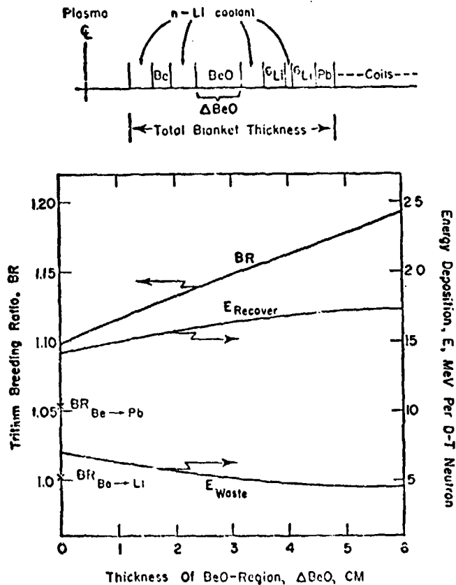
FIGURE 1. Tritium breeding and energy recovery of thin (21.8 cm with \Delta\text{BeO}=0 ) RTPR blanket (MOD-1) vs thickness of beryllium oxide region.
