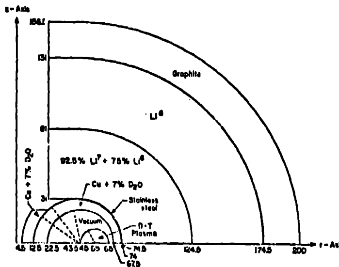
Fig. 1. Two-dimensional RIGGATRON (dimensions in cm).
