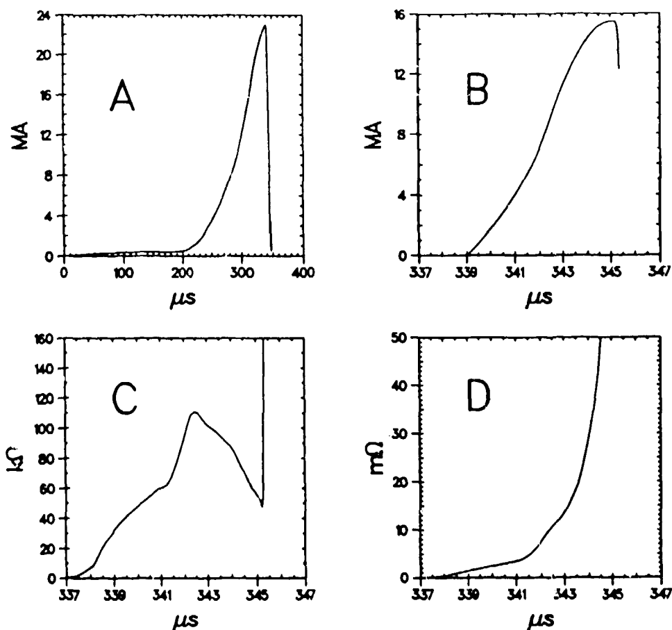
Fig. 2. Calculated (A) total current profile, (B) plasma gun current, (C) driving voltage and, (D) extrapolated switch resistance for EFF version.
