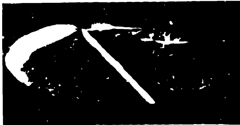
Fig. 4b. IIC photo of welded plate showing emerging jet at 0.5 \mu s after fiducial.
