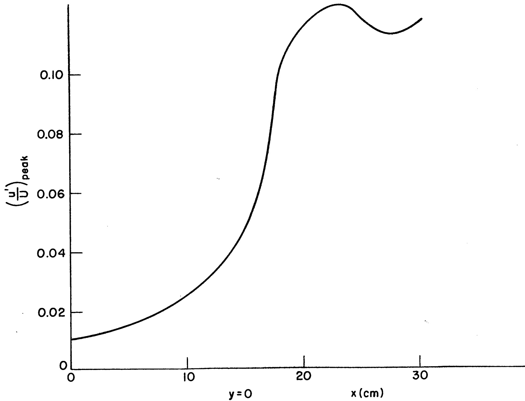
Fig. 7. Downstream variation of peak disturbance amplitude. At x=0 (upstream boundary), disturbance is 1% two-dimensional Tollmien-Schlichting wave with .15% three-dimensional perturbation.
