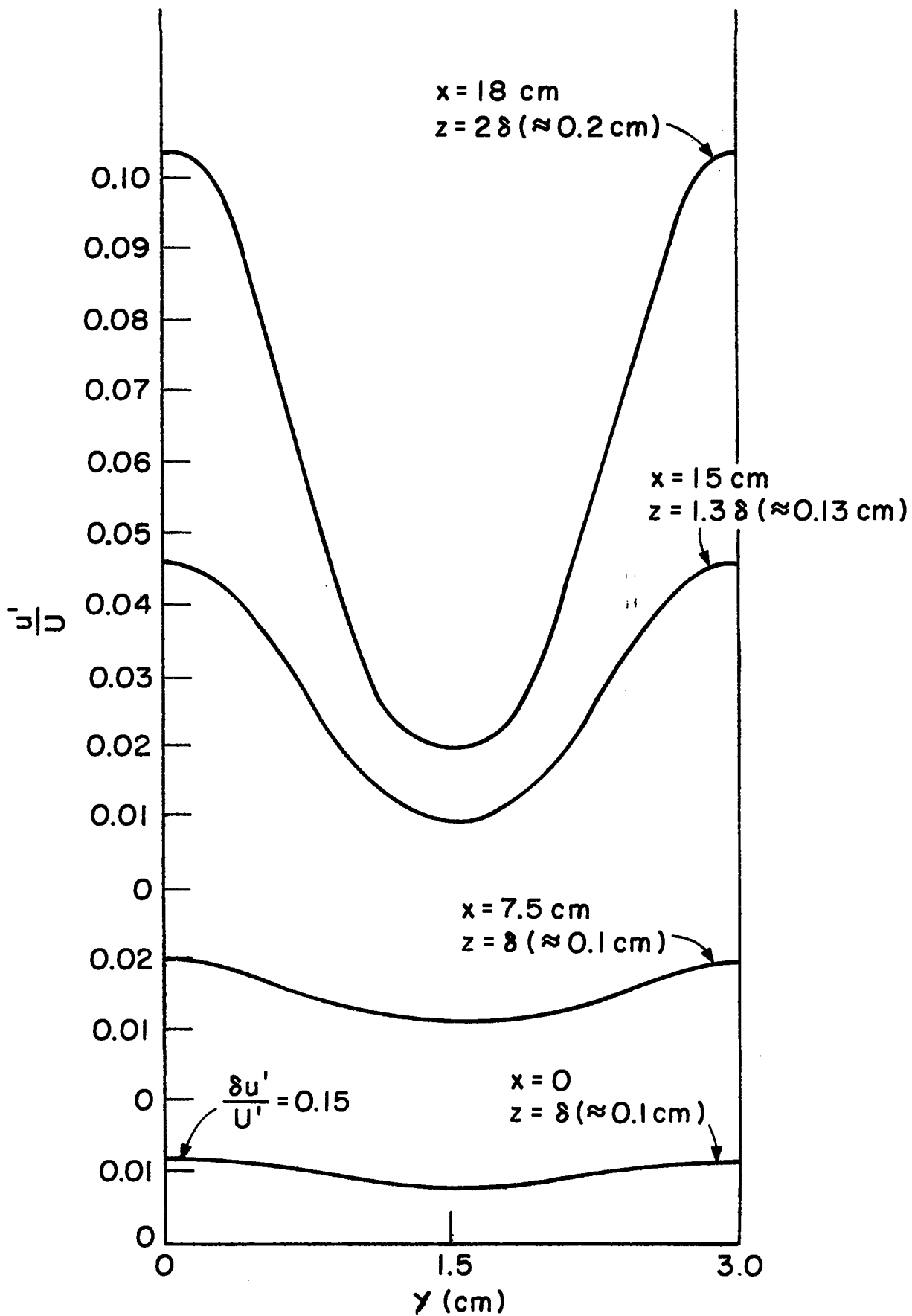
Fig. 8. Cross-stream ( y ) variation of disturbance amplitude for several downstream ( x ) locations.
