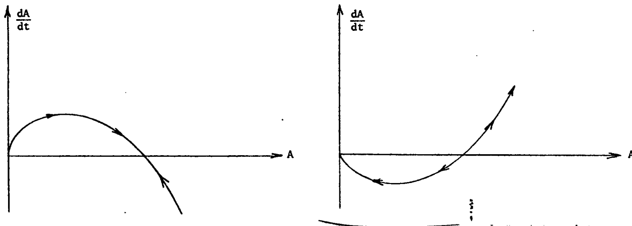
Fig. 2. Phase plane behavior of finite amplitude disturbances
