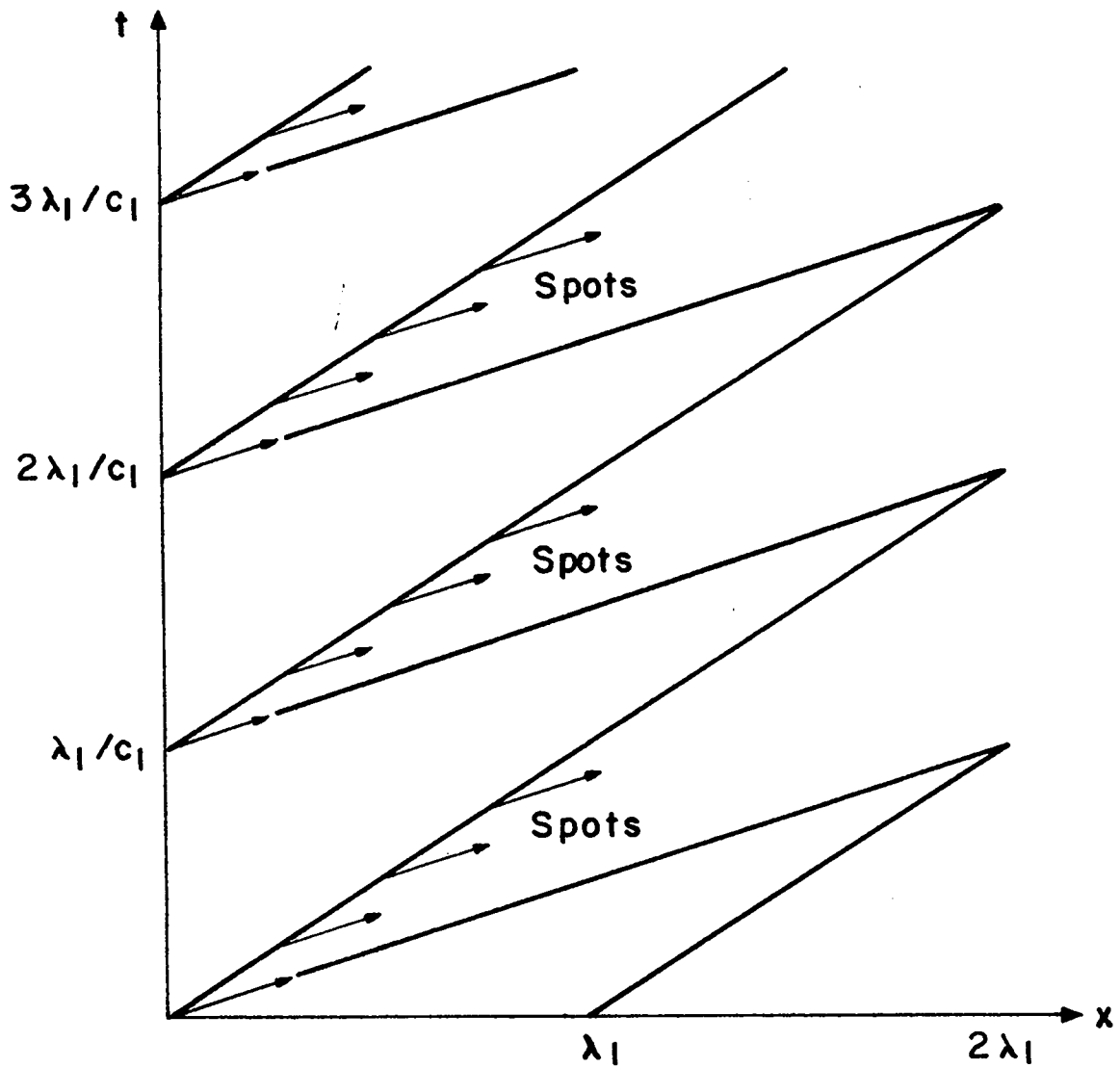
Fig. 5. x - t representation showing favorable locations for onset of secondary instability.
