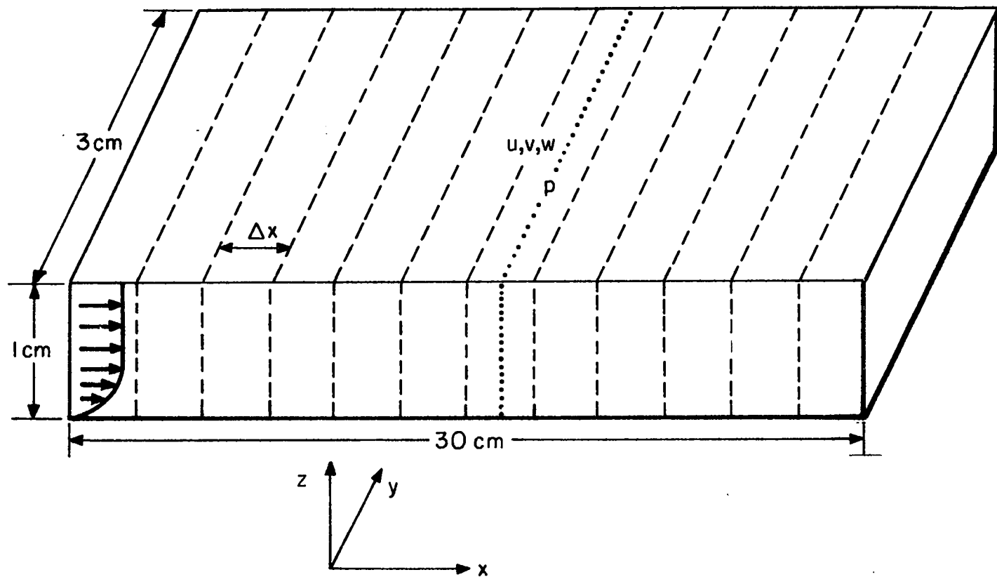
Fig. 6. Computational domain for transition experiments: \Delta x = 30 \text{ cm}/128 , 8 Fourier modes in y , 65 Chebyshev polynomials in z . Inflow conditions: \delta = \sqrt{\nu X/U} \approx .1 \text{ cm} , U \approx 1500 \text{ cm/s} , R \approx 10^3 , X \approx 100 \text{ cm} .
