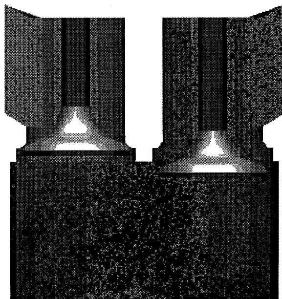
Fig. 3.1-1. A color visualization of the temperature field during the inlet flow in a hydrogen-fueled engine simulated with KIVA-3 [62][90]. The open intake valve is on the right; the closed exhaust port is on the left. The particles are used only to simulate the flow and are colored according to the temperature of the gas. The cold intake air (blue) is shown compressing the residual hot combustion gases (red).
