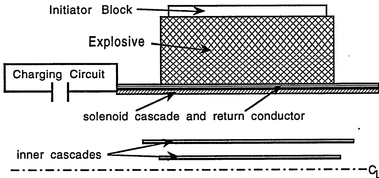
Fig. 1. Diagram of the Russian three-cascade MC-1 FCG.
