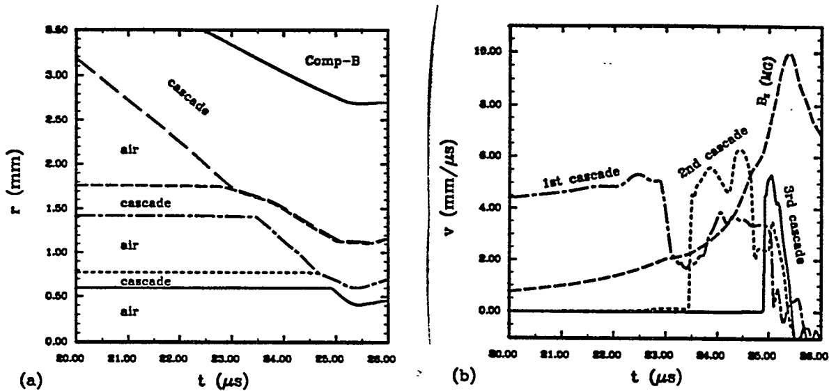
Fig. 2. Cascade radii (a) and velocity (b) for Comp-B simulations using the mixed EOS. Calculated field is overlaid in (b).
