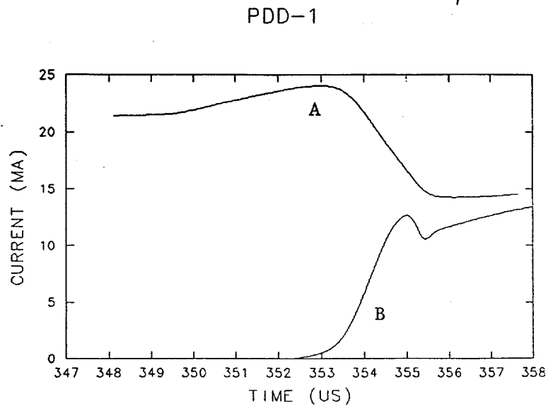
Figure 4. Storage inductor (A) and load (B) currents for test producing 1.5 MJ radiation. The dip at \sim 355 \mu\text{s} indicates pinch occurring.
