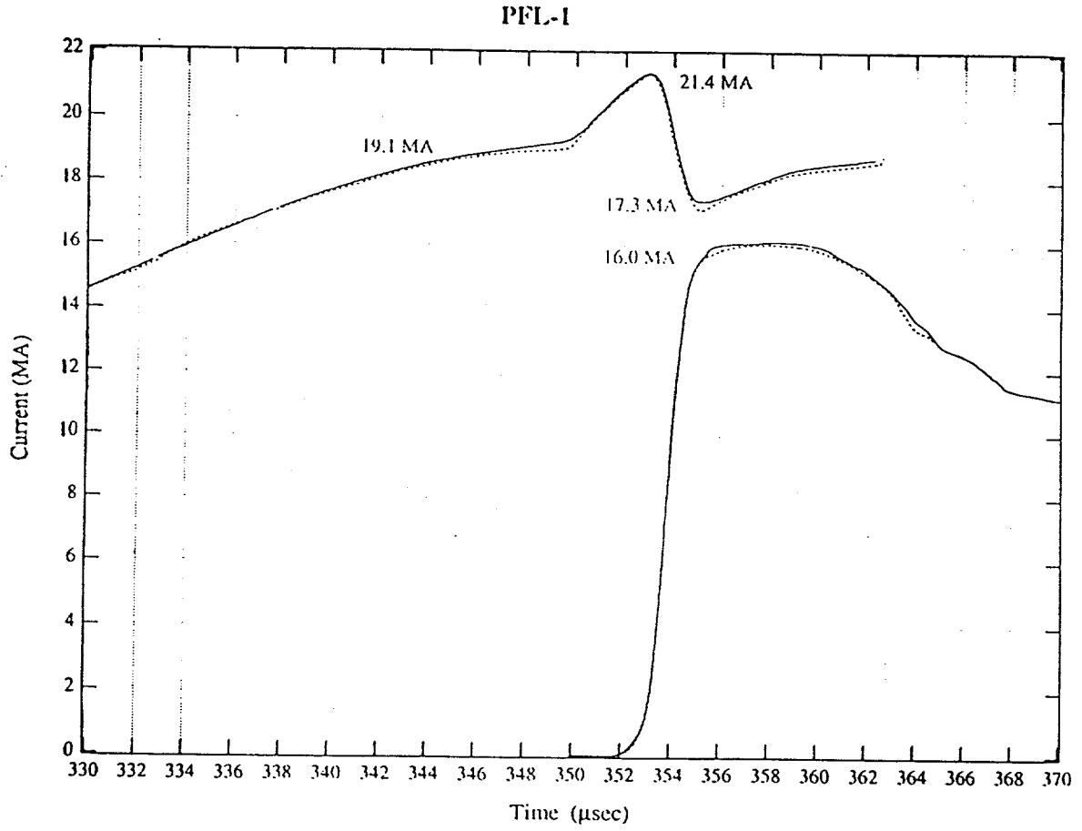
Figure 8. Storage (A) and load (B) currents for our first Procyon Liner Experiment. Implosion begins to affect the waveform at ~ 360 μs.
