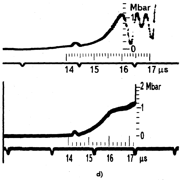
Fig. 3. Processed Oscillograms of Induction, Manganese, and X-ray Probes Signals. a) cable length calibration; b) compression onset; c) X-ray exposure; d) piezoresistive technique signals
