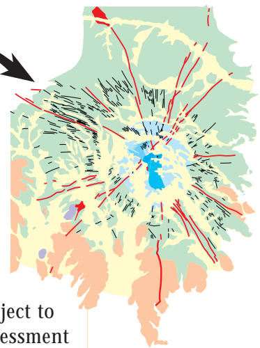
Summer Coon Volcano, Colorado (32 million years old)
