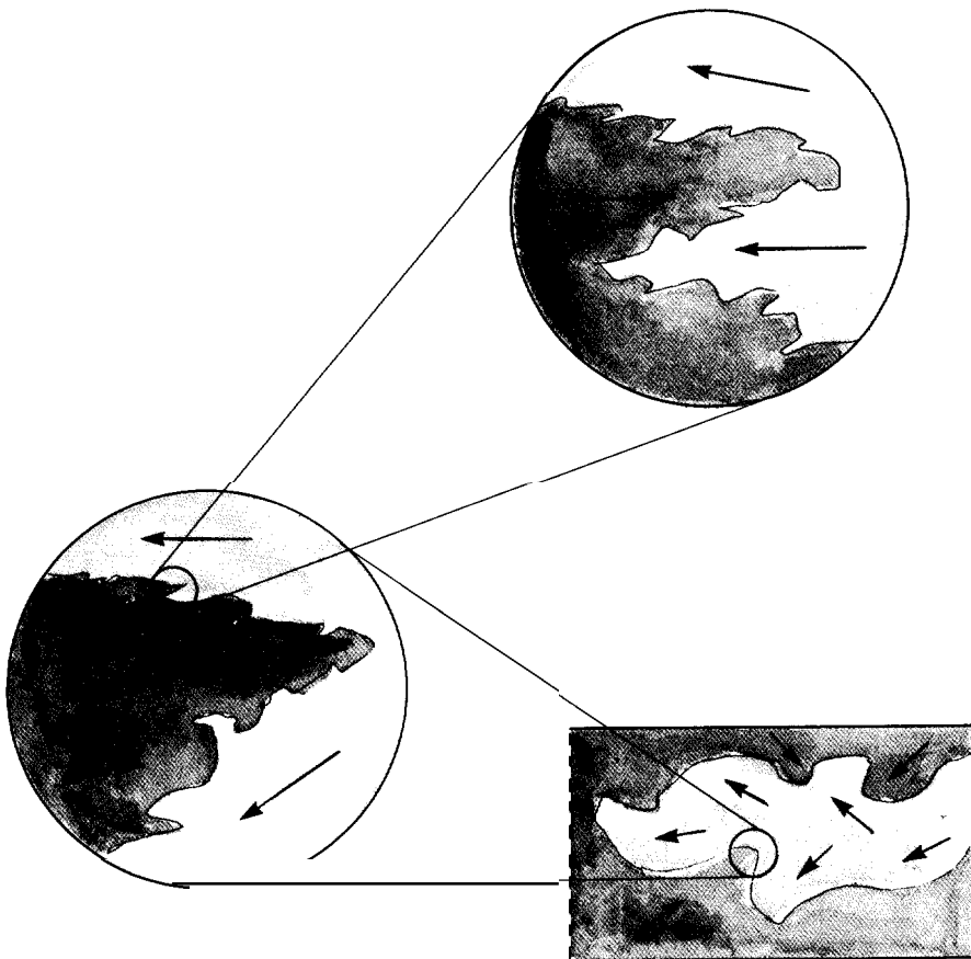
Fig. 8. With each reduction in scale, turbulent motion of the larger scale becomes mean-flow motion of the smaller scale (arrows). Because each reduction in scale has approximately the same change in mean-flow velocity occurring over a much smaller distance, velocity gradients become steeper, and a larger fraction of the turbulence energy goes directly into heat.
