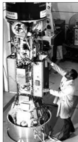
A researcher checks the radio-frequency power amplifiers of the Beam Experiment Aboard a Rocket, or BEAR, which was the first U.S. test of a neutral particle beam in space.
