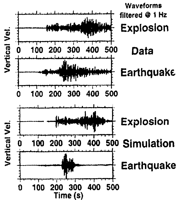
Figure 2. Crustal structure between Lop Nor and station AAK (above), located ca. 1200 km W of Lop Nor; earthquake and explosion waveforms at this station (right). There is approximate qualitative agreement between the data and simulation for both sources. The simulations exhibit a lack of Lg coda, likely due to a lack of scattering in the 2-D calculations.
