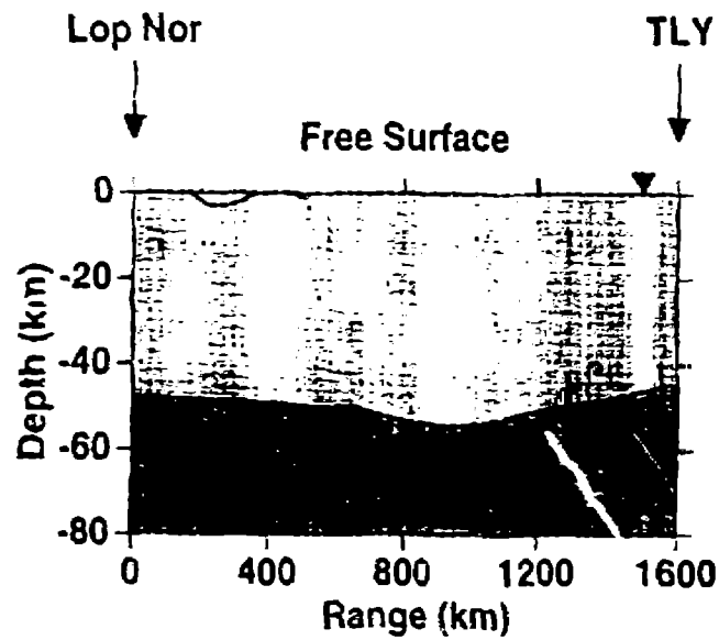
Figure 4. Crustal structure between Lop Nor and station TLY (above), located ca. 1600 km NE of Lop Nor; earthquake and explosion waveforms at this station (right). The path exhibits a mildly varying Moho and minor sedimentary basin. There is approximate qualitative agreement between the data and simulation for both sources, with the exception of the weak Lg coda in the simulations.
