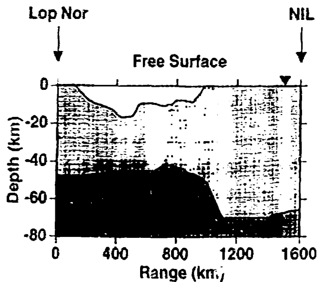
Figure 3. Crustal structure between Lop Nor and station NIL (above), located ca. 1600 km SW of Lop Nor; earthquake and explosion waveforms at this station (right). The path exhibits a strongly dipping Moho as well as a pronounced sedimentary basin. There is approximate qualitative agreement between the data and simulation for both sources.
