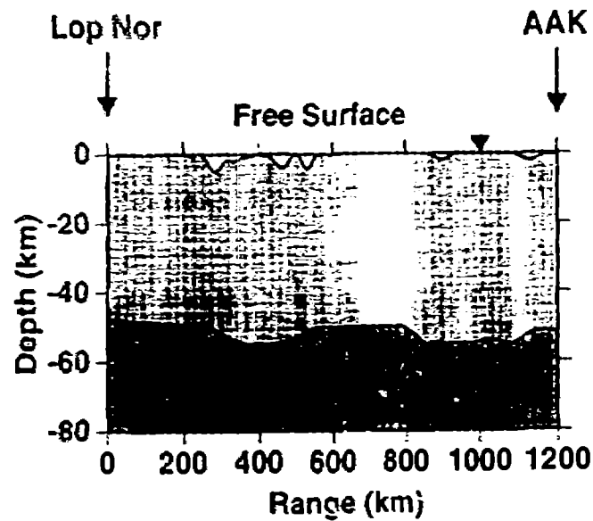
Figure 2. Crustal structure between Lop Nor and station AAK (above), located ca. 1200 km W of Lop Nor; earthquake and explosion waveforms at this station (right). There is approximate qualitative agreement between the data and simulation for both sources. The simulations exhibit a lack of Lg coda, likely due to a lack of scattering in the 2-D calculations.
