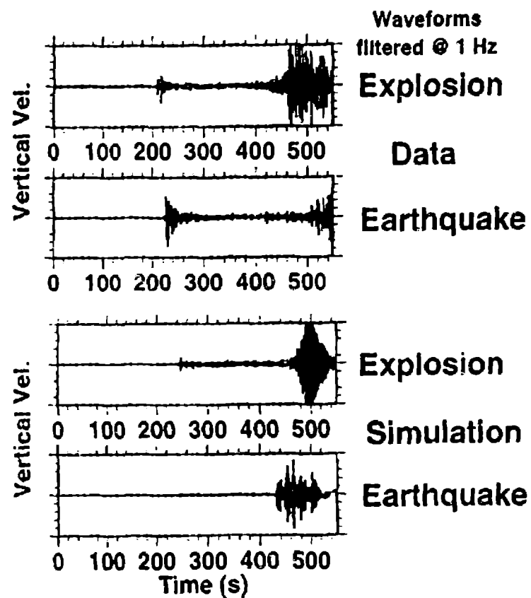
Figure 5. Crustal structure between Lop Nor and station ULN (above), located ca. 1600 km ENE of Lop Nor; earthquake and explosion waveforms at this station (right). The path is similar to that to station TLY (Fig. 4). There is notable disagreement between the data and simulation for these sources: the data for both the earthquake and explosion show a distinctive P_g that is lacking in the corresponding simulations.
