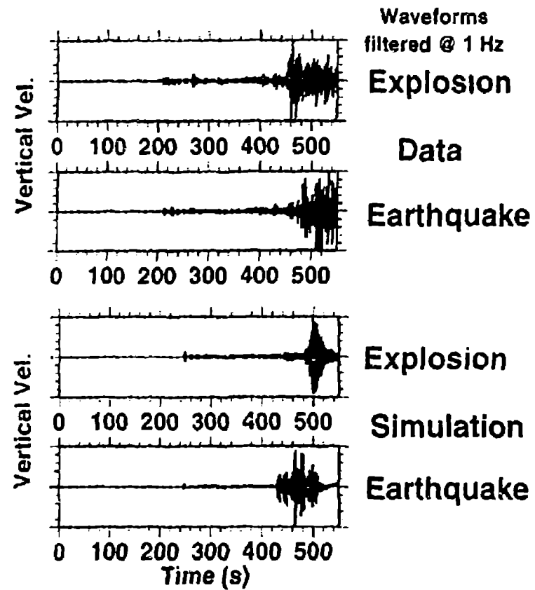
Figure 4. Crustal structure between Lop Nor and station TLY (above), located ca. 1600 km NE of Lop Nor; earthquake and explosion waveforms at this station (right). The path exhibits a mildly varying Moho and minor sedimentary basin. There is approximate qualitative agreement between the data and simulation for both sources, with the exception of the weak Lg coda in the simulations.
