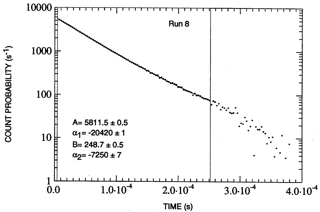
Fig. 5. Rossi- \alpha curve at approximately -0.55. The data was accumulated for approximately 5 hours. The LSF was performed in the time interval between the origin and the vertical line drawn at 2.5 \times 10^{-4} s. The data to the right of the vertical line has been affected by the large intrinsic source strength.
