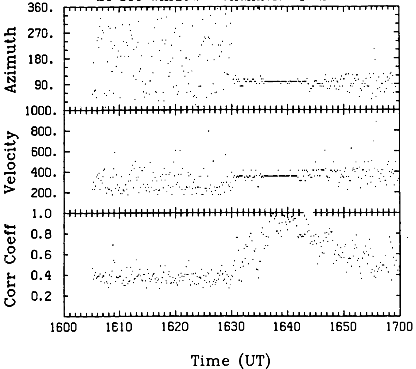
Figure 2. Summary of beamformer array processing program showing correlation coefficient, trace velocity, and azimuth as functions of time. Data are for Miser's Gold event observed at Reedley, Ca.
