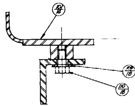
SECTION A-A TYPICAL
