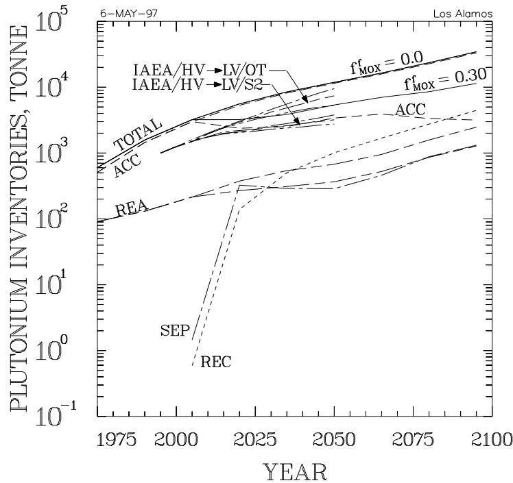
Figure 9. Time dependence of global plutonium inventories by form for a MOX core (volume) fraction of 0.30 beginning in \sim 2005 and taking 25 years to reach this asymptote. ACC = plutonium accumulated in spent fuel form that can undergo recycle back to the LWR; REC = plutonium that has experienced the maximum ( N = 3 ) recycles; REA = average plutonium inventoried in reactors; SEP = separated plutonium in MOX fuel fabrication and chemical processing; TOTAL = ACC + REC + REA + SEP.
