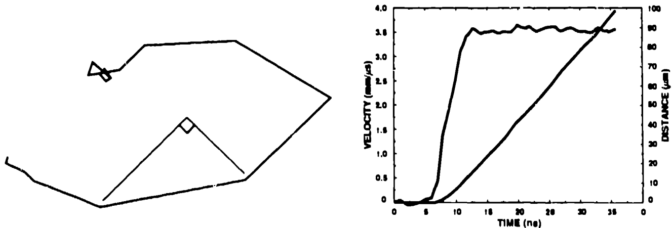
Figure 3: VISAR Lissajous and reduced velocity profile from data recorded with PMT/digitizer system at ~2–3 ns/pt.
