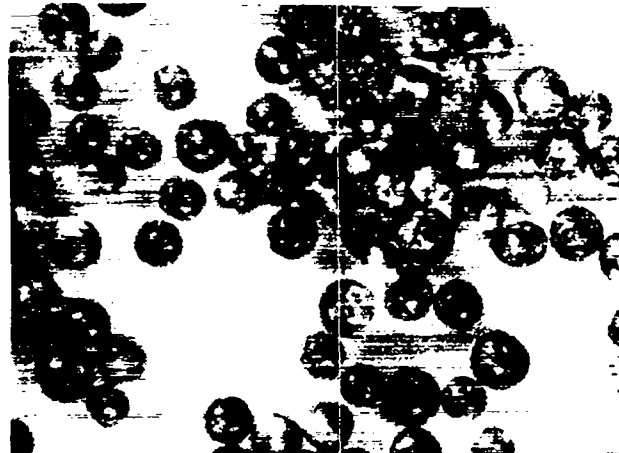
As-spheroidized at 1150°C in argon atmosphere, \text{D}_2 content 19.34 wt%.
