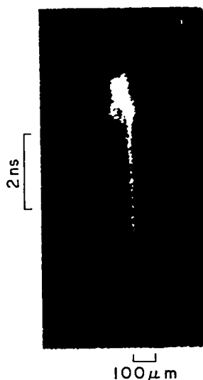
Fig. 5. Streak-camera data at high magnification ( \times 33 ). Time increases from top to bottom.
