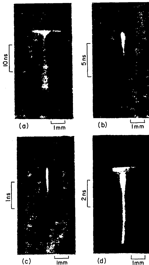
Fig. 4. Streak-camera data at low magnification ( \times 5.5 ) showing the time dependence of the light emerging from the backs of four 13- \mu\text{m} -thick aluminum targets after each was struck by a 100- \mu\text{m} -diam, 300-ps laser pulse of about 35 J. The streaks run from top to bottom. They show an intense light pulse that lasts for about 0.8 ns and is followed by a dimmer light lasting for at least 25 ns. Figure 4d is overexposed, exaggerating the initial bright pulse but clearly showing the first 6 ns of the tail.
