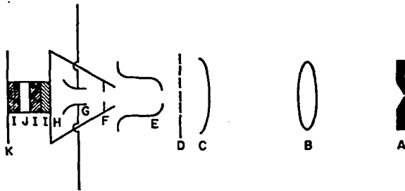
Fig. 3. Schematic of the streak camera: A) object slits; B) internal lens; C) photocathode; D) grid; E) focus electrode; F) anode; G) deflection plates; H) fluorescent screen; I) fiber-optical couplers; J) image intensifier; K) film. Elements C through H are contained in the image tube.
