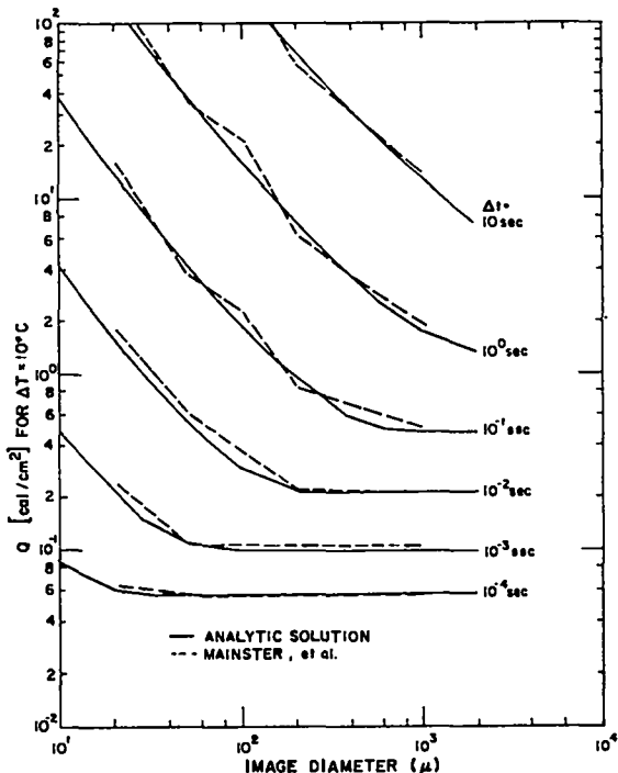
Fig. 1. Comparison of the analytic solutions to the numerical solutions of Mainster et al. 1 for various values of R_0 and t . Monochromatic 7000\text{-}\text{\AA} source.
