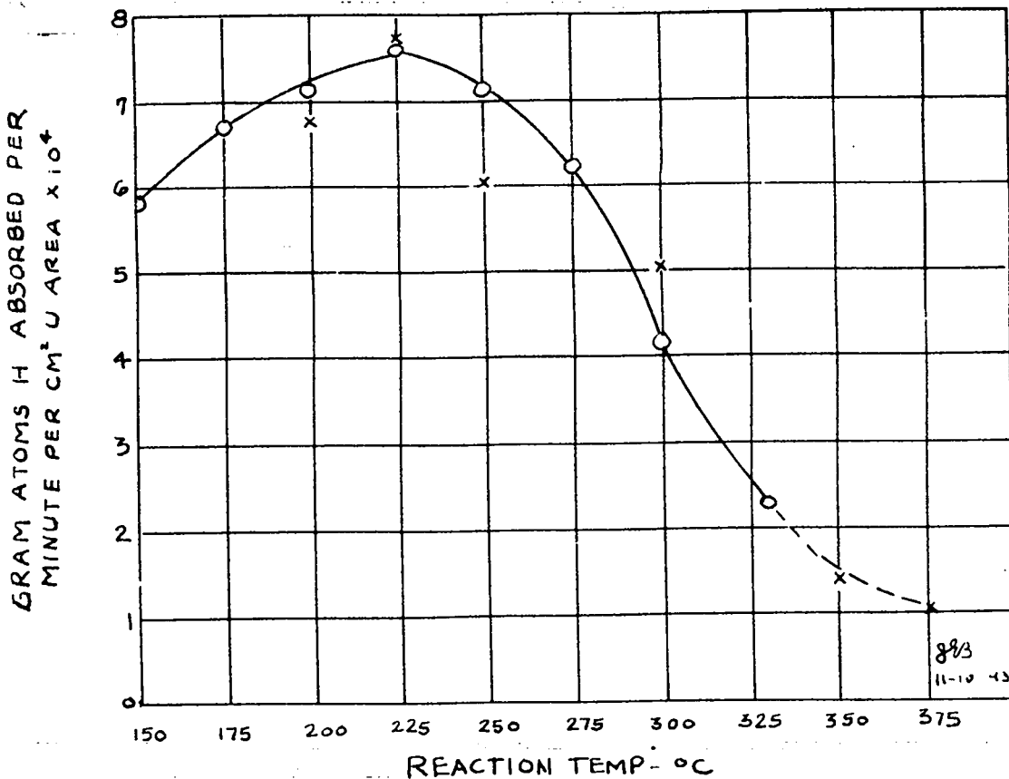
EFFECT OF TEMPERATURE ON REACTION RATE
