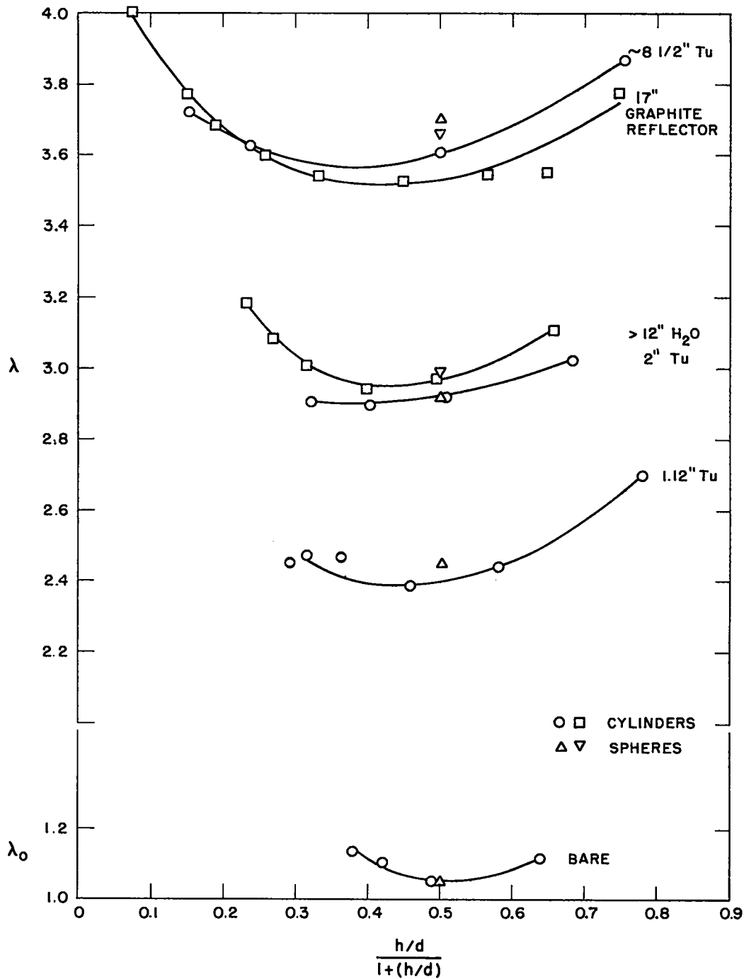
Fig. 5 Curve of \lambda vs. (h/d)/(1 + h/d) with \lambda_{OS}(\text{sphere}) \equiv 1.05 \text{ cm.}
