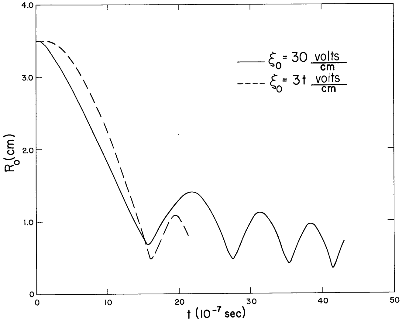
Fig. 3 Hydrodynamic solution of pinch equations. Radius as a function of time t for the two values of \xi_0 indicated. In both problems \rho_0 = 2.041 \times 10^{-8} gms/cc; radius of conductor = 3.86 cm.
