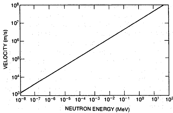
Fig. 12.1 Graph showing the relationship between a neutron's speed and its kinetic energy.
