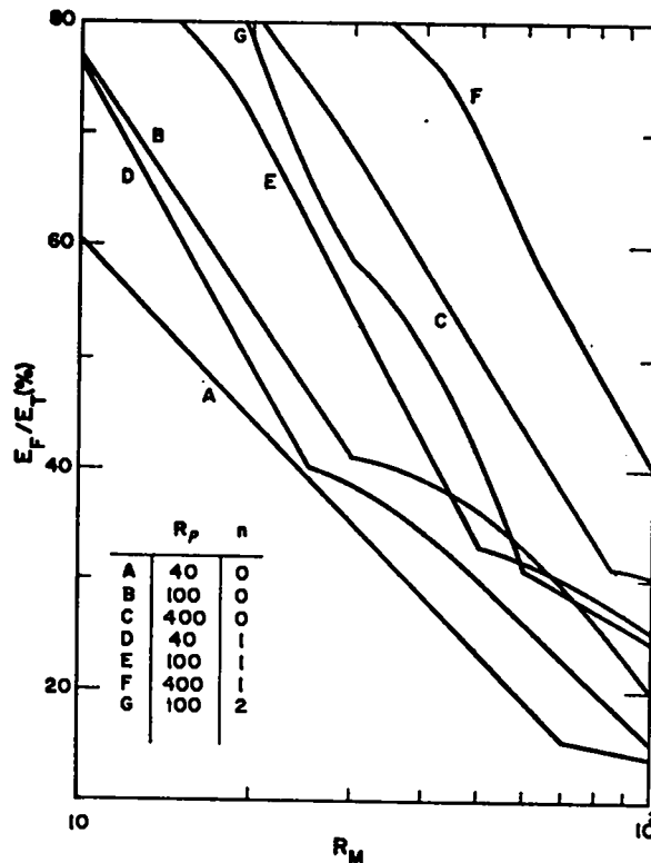
Fig. 3. Transfer efficiency.
