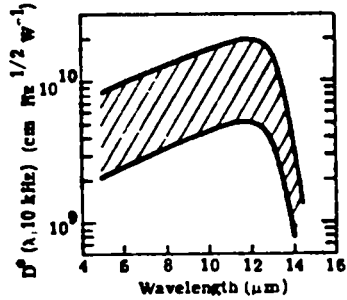
(a) Spectral response of detector D^* ( \lambda, 10 \text{ kHz} ).
