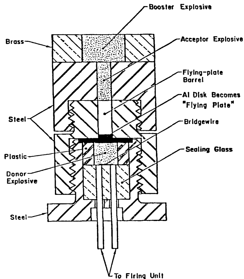
Fig. 1. Flying-plate assembly.
