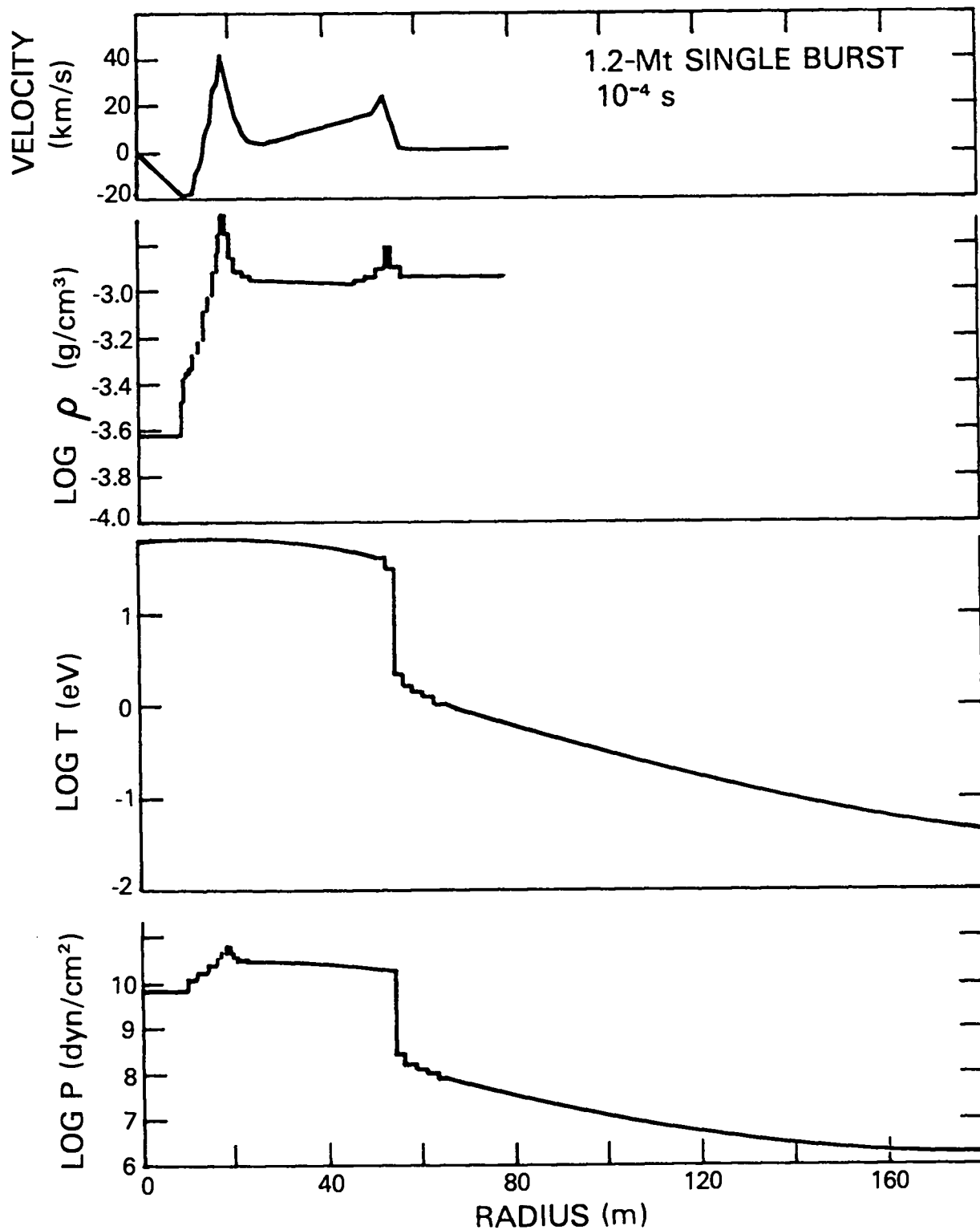
Fig. 1. Flow-field profiles at 0.1 ms for the first 1.2-Mt burst computed with RADFLO. The hydrodynamic shockwave has just begun to form near 56-m radius.
