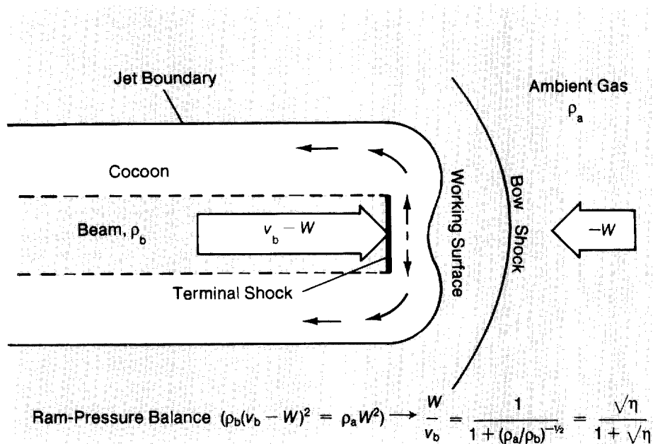
Fig. 6. Flow schematic of the jet head in the rest frame of the working surface. The speed of advance W of the working surface is determined by equating the ram pressure, or momentum flux, of the beam to the ram pressure of the ambient gas in a frame in which the working surface is stationary. In this frame the beam speed is v_b - W and the speed of the ambient gas is -W . The expression derived for W/v_b implies that, for jets with low density ratios ( \eta \ll 1 ), the working surface advances much more slowly than the beam gas. However, the beam gas does not collect at the working surface but is shock decelerated and deflected sideways to form a low-density backward flowing cocoon around the forward moving beam.
