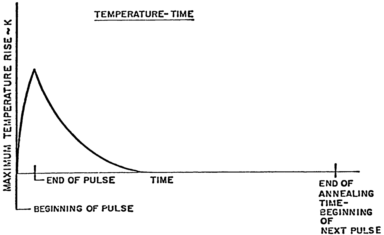
Figure 2. Schematic of the temperature - time profile of a metal foil under pulsed irradiation at the foil mid-plane and at the center of a Gaussian beam spot.
