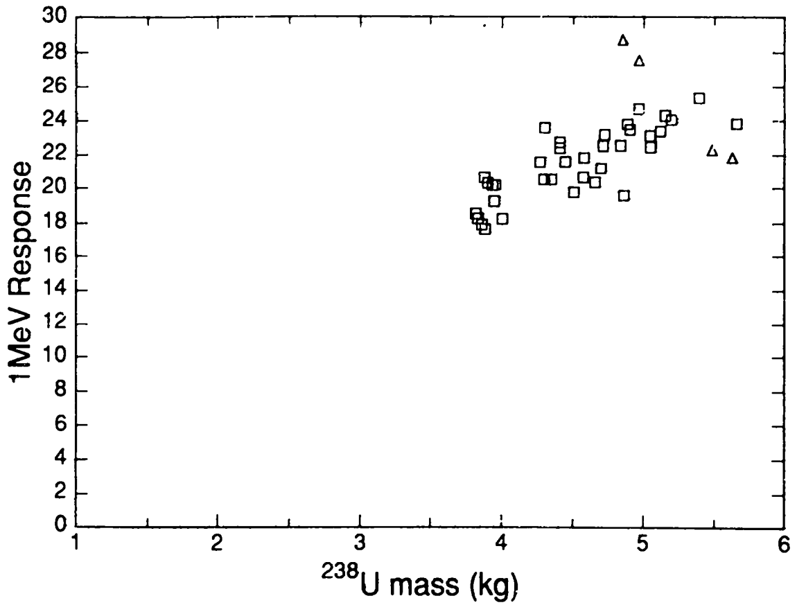
Fig. 10. Plot of ^{238}\text{U} mass vs count rate for 41 samples of the same chemical form. Note four anomalous points (designated by \Delta ) caused by interchanged mass values.
