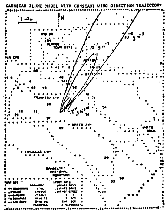
Fig. 2. Results of Gaussian plume calculations for nominal plume case.
