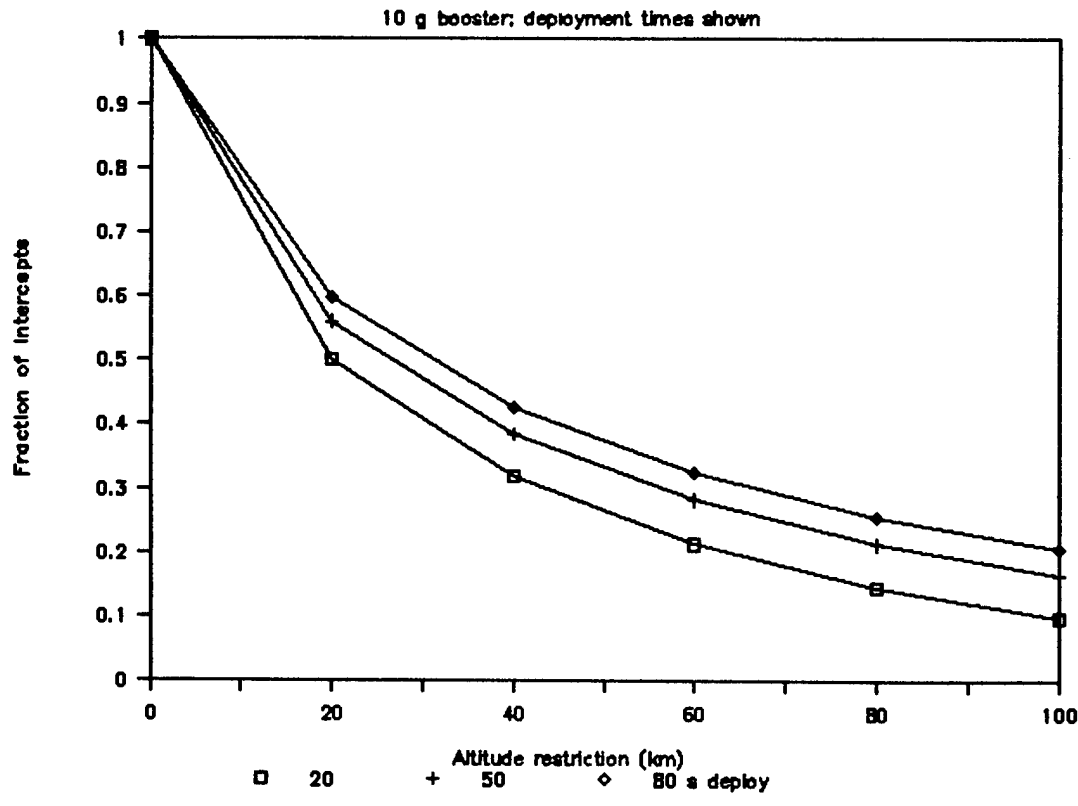
Fig. 2. Penalty for altitude and shielding.
