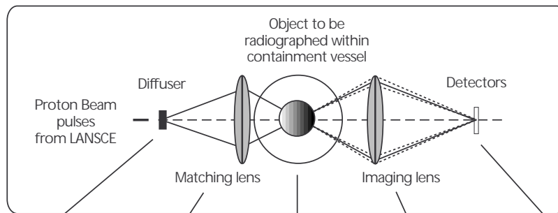
Optical analogy of magnetic lens system (vertical dimensions greatly expanded)
