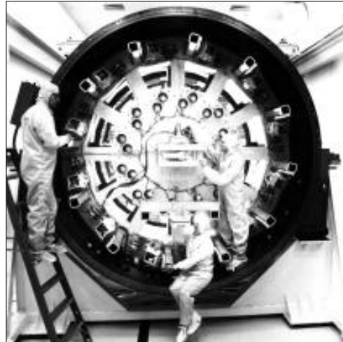
This 10-foot-diameter optical spool expanded and relayed beams from Antares, a carbon-dioxide laser system built to investigate whether such a system could initiate inertially confined fusion.
